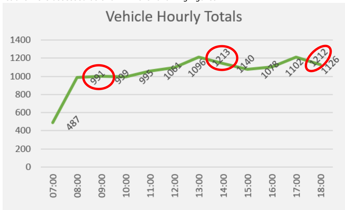
Figure 4.3 Network Traffic Profile for AM & 2x PM Peak Flows
