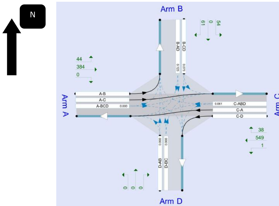
Figure 6.1: Junction 1 - Development Junction
