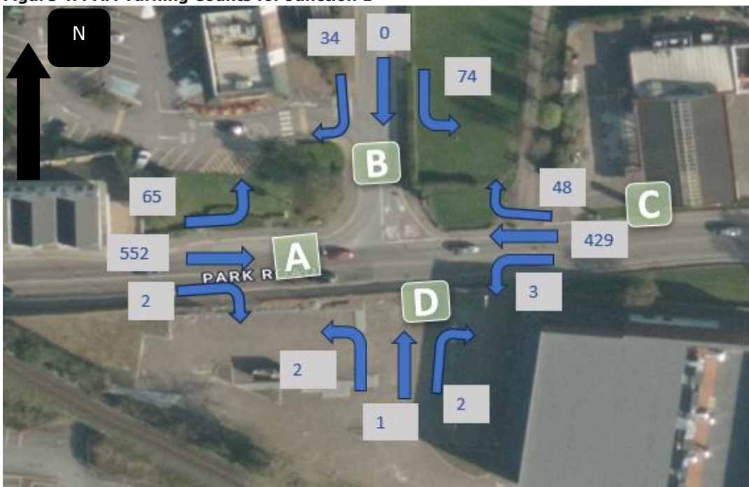
Figure 4.5 PM Turning Counts for Junction 1
